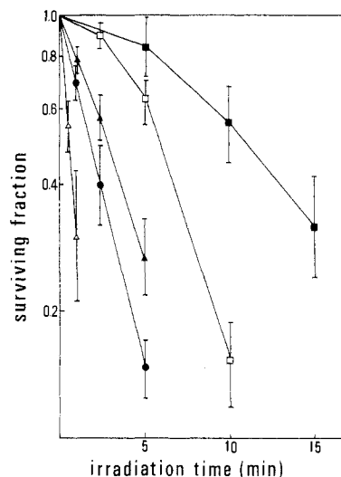
Figure 3. Inactivation of T_2 phage by irradiation (365 nm) in the presence of 2a (▲), 2b (●), 2c (△), 1 (■), and 8-methoxypsoralen (8-MOP) (□). After irradiation, the plaque forming per milliliter were scored by using E. coli B 48 as indicator bacteria. Incubation in the dark in the presence of the drugs and 40-min irradiation in their absence were both unable to reduce significantly the surviving fraction.
