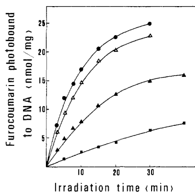
Figure 2. Photobinding of 2a (▲), 2b (●), 2c (△), and 1 (■), as reference compound, toward calf thymus DNA.
